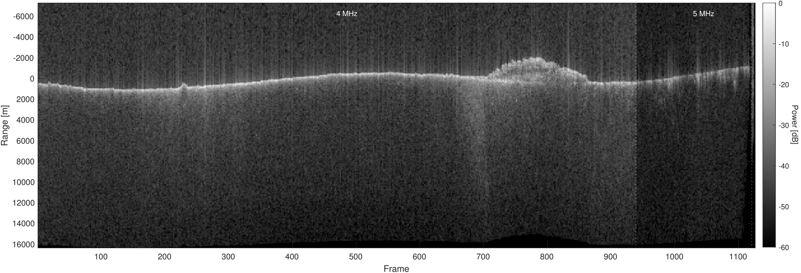
Orbit 11985, Optimized, No Window, Depth-Corrected, Channel 2
