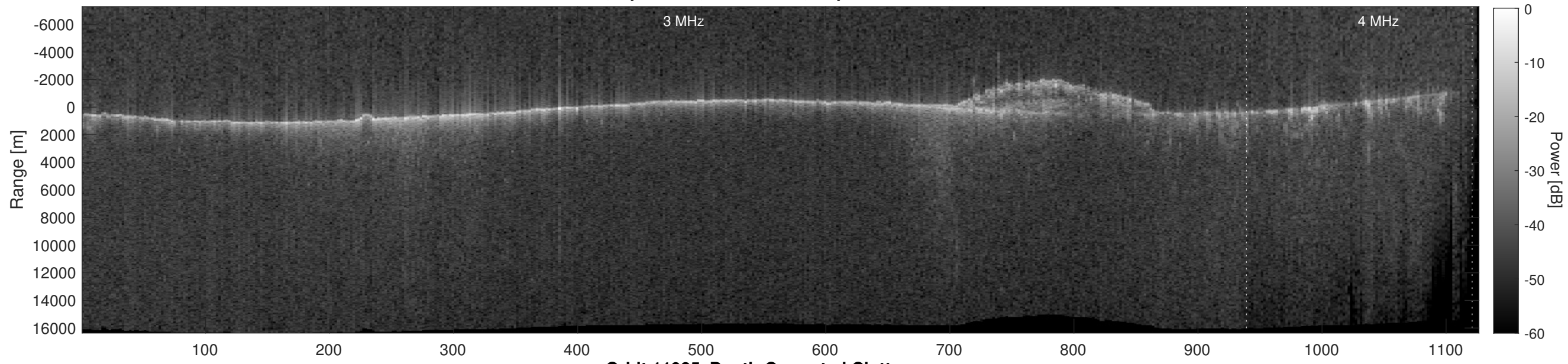
Orbit 11985, Depth-Corrected Cluttergram
