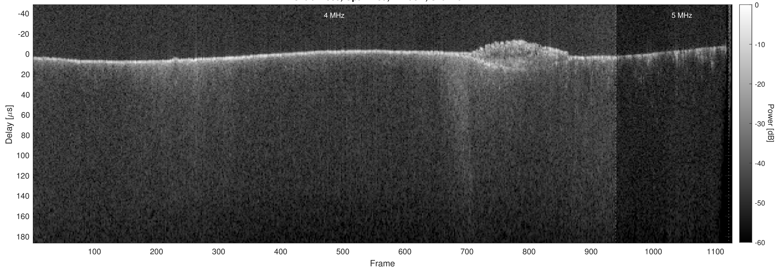
Orbit 11985, Optimized, Window, Channel 2
