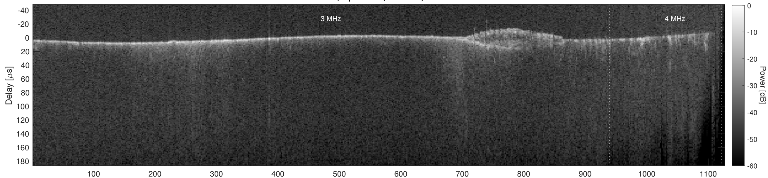
Orbit 11985, Cluttergram
