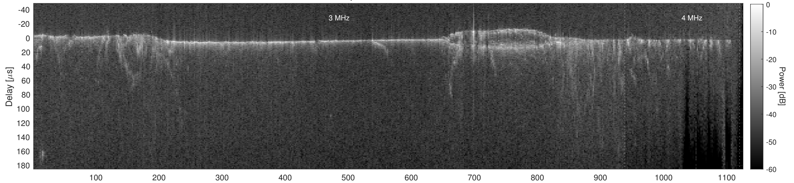
Orbit 11986, Cluttergram
