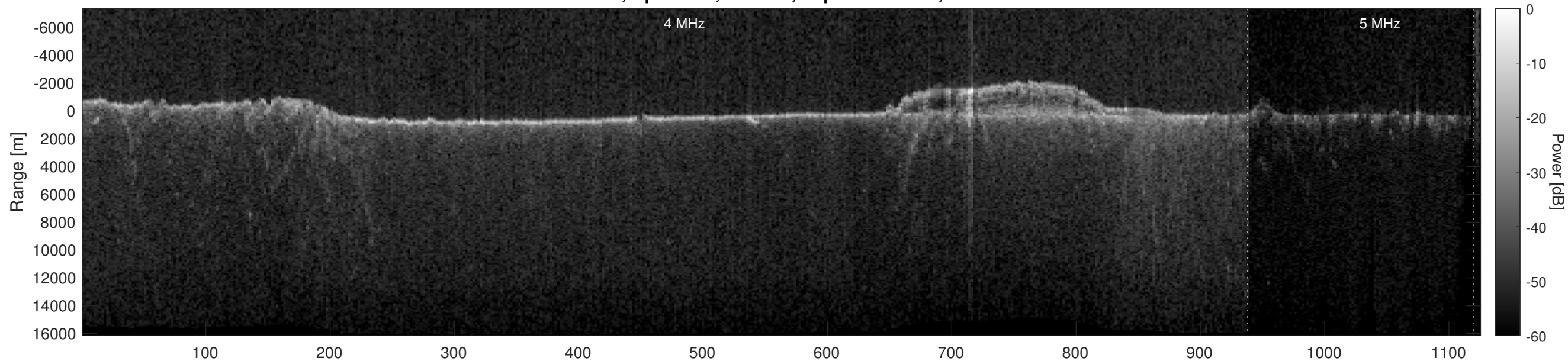
Orbit 11986, Optimized, Window, Depth-Corrected, Channel 2
