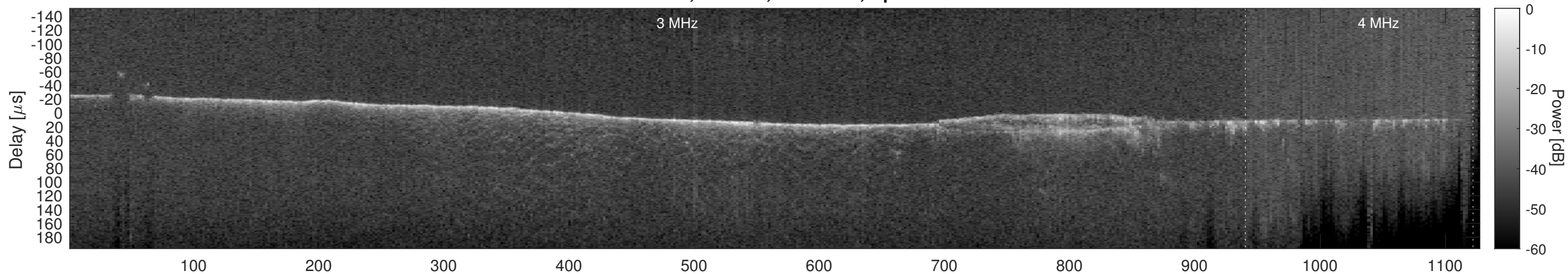
Orbit 11987, Cluttergram
