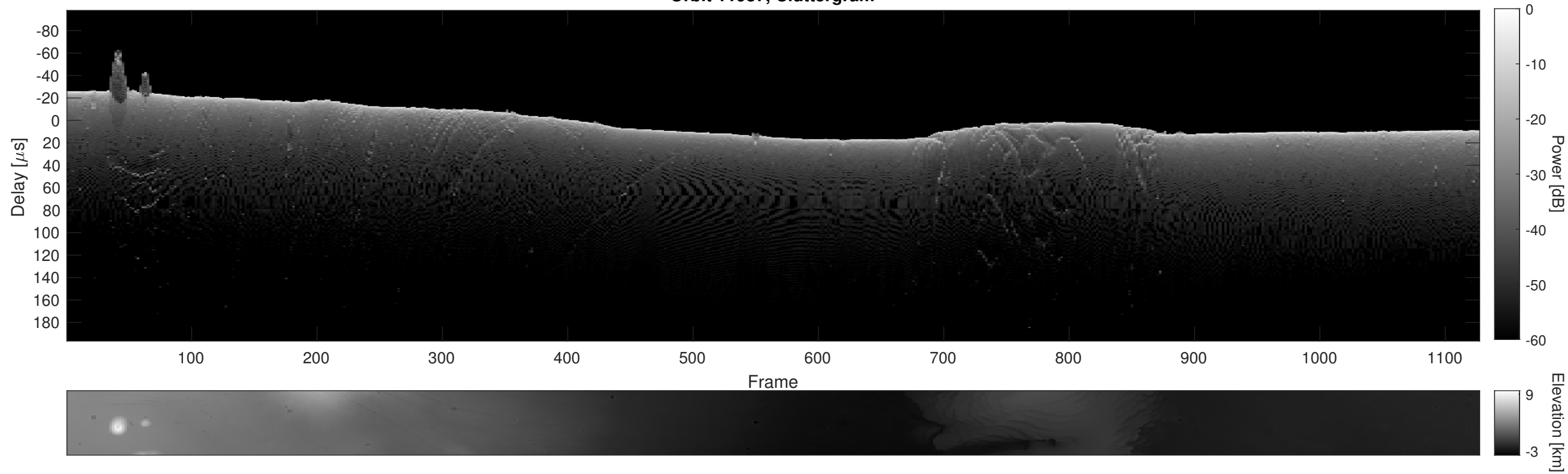
Orbit 11987, Cluttergram
