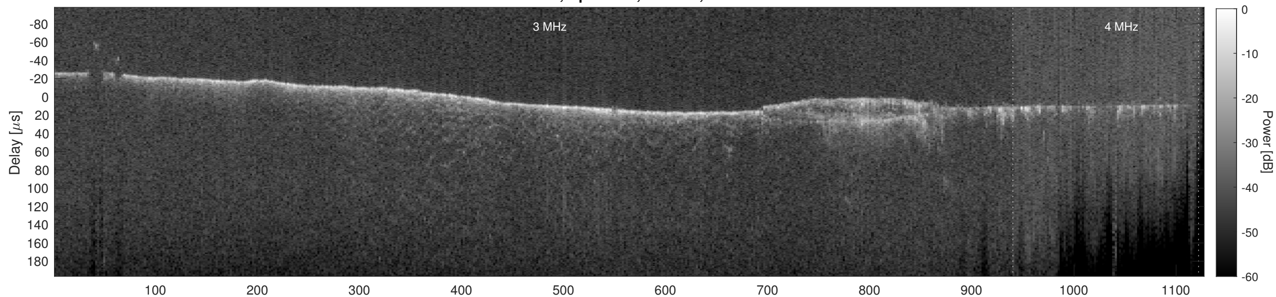
Orbit 11987, Cluttergram
