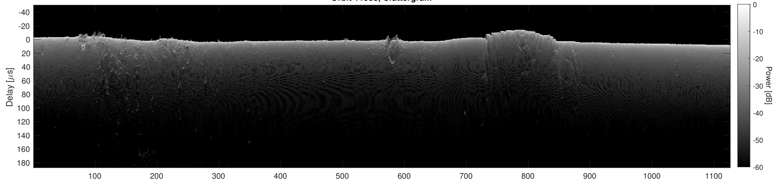
Orbit 11988, Cluttergram
