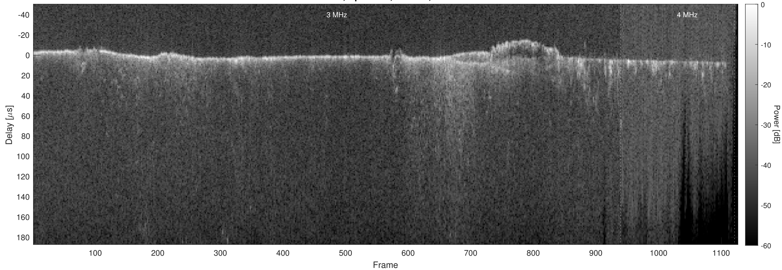
Orbit 11988, Optimized, Window, Channel 2
