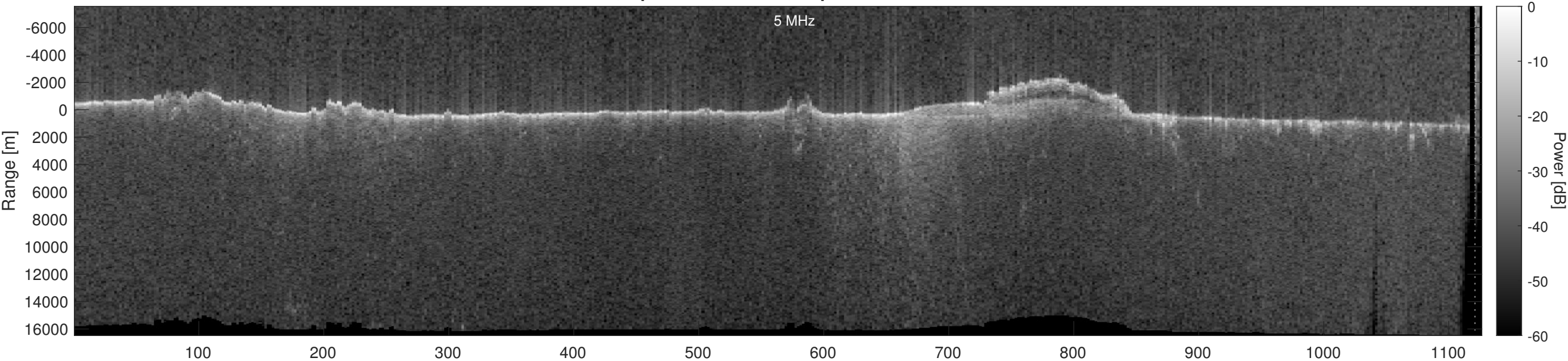
Orbit 11988, Optimized, Window, Depth-Corrected, Channel 2
