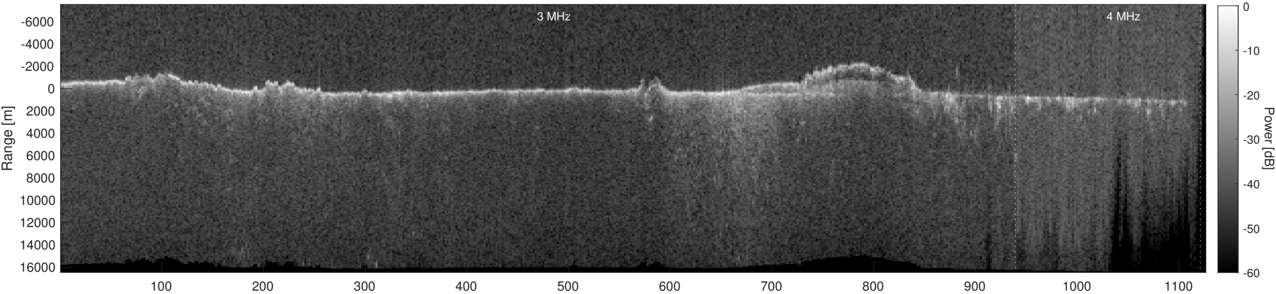
Orbit 11988, Depth-Corrected Cluttergram
