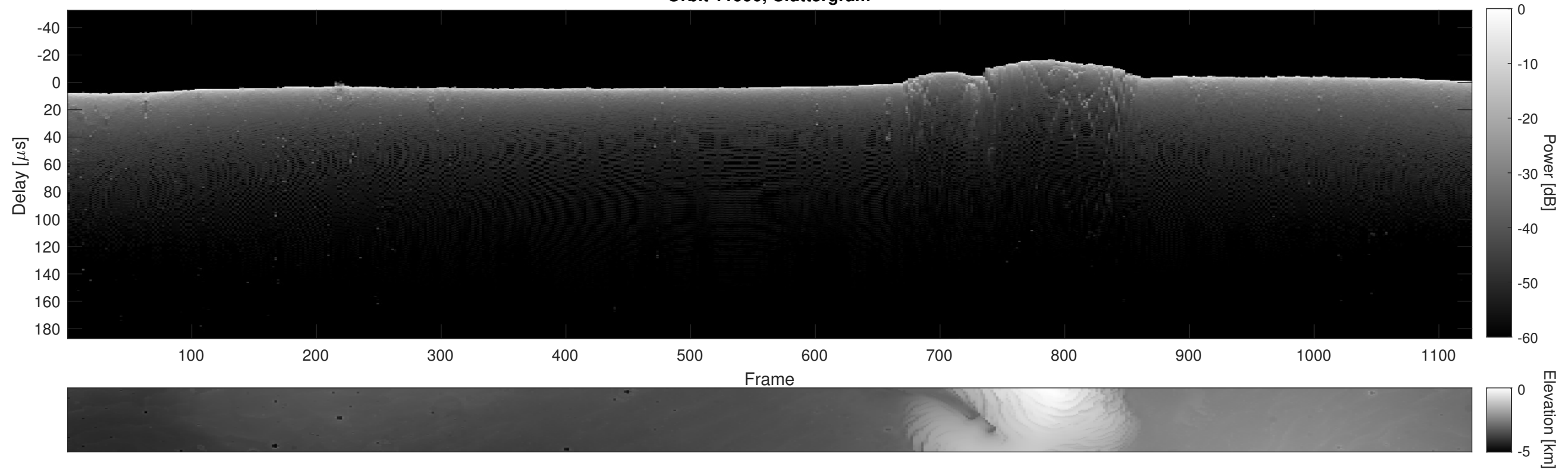
Orbit 11990, Cluttergram
