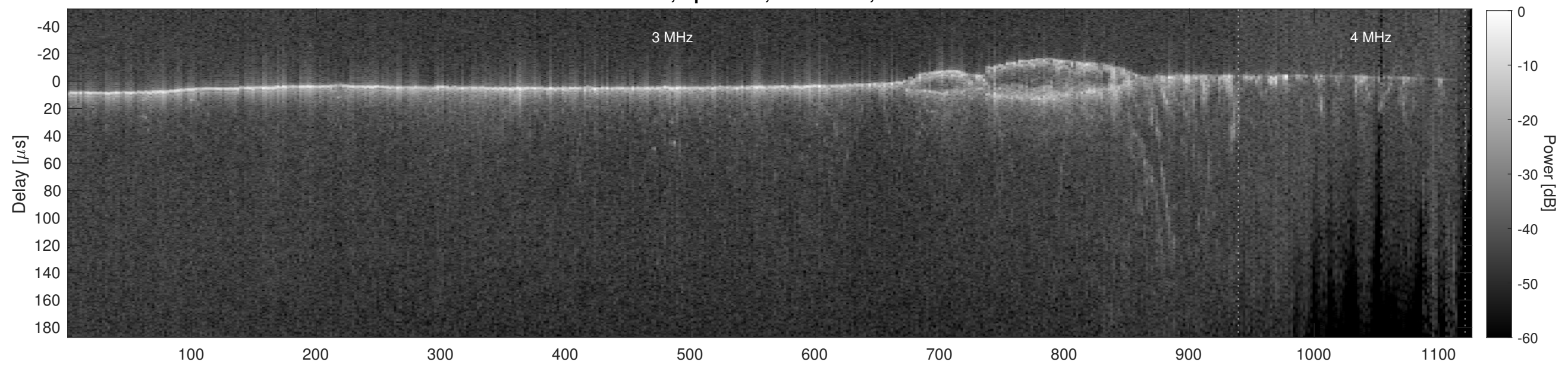
Orbit 11990, Cluttergram
