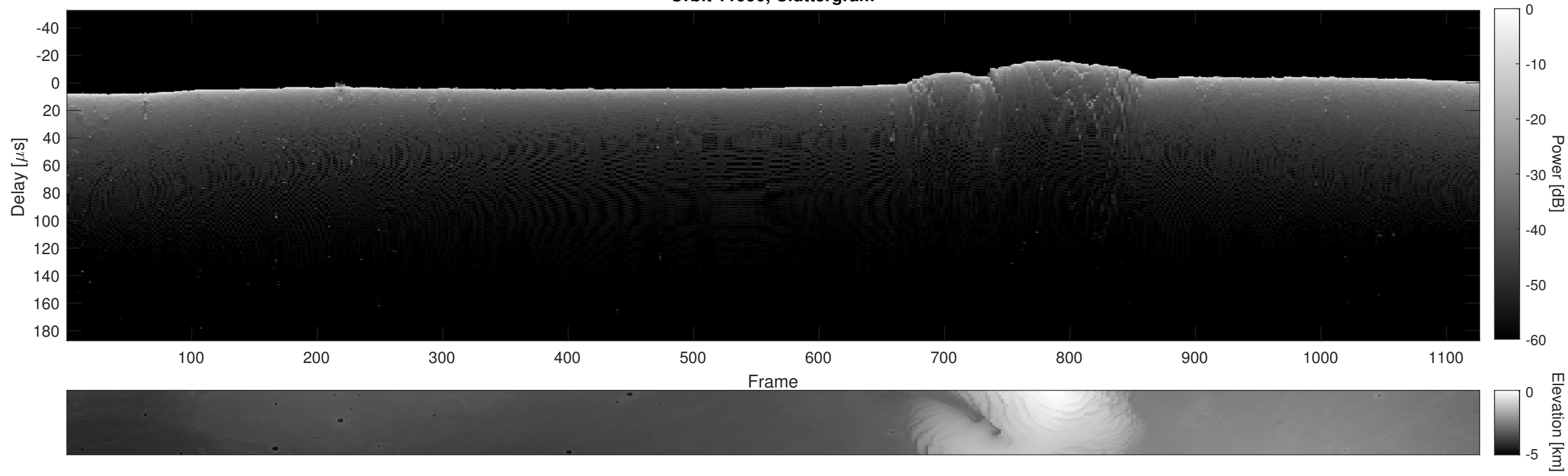
Orbit 11990, Cluttergram
