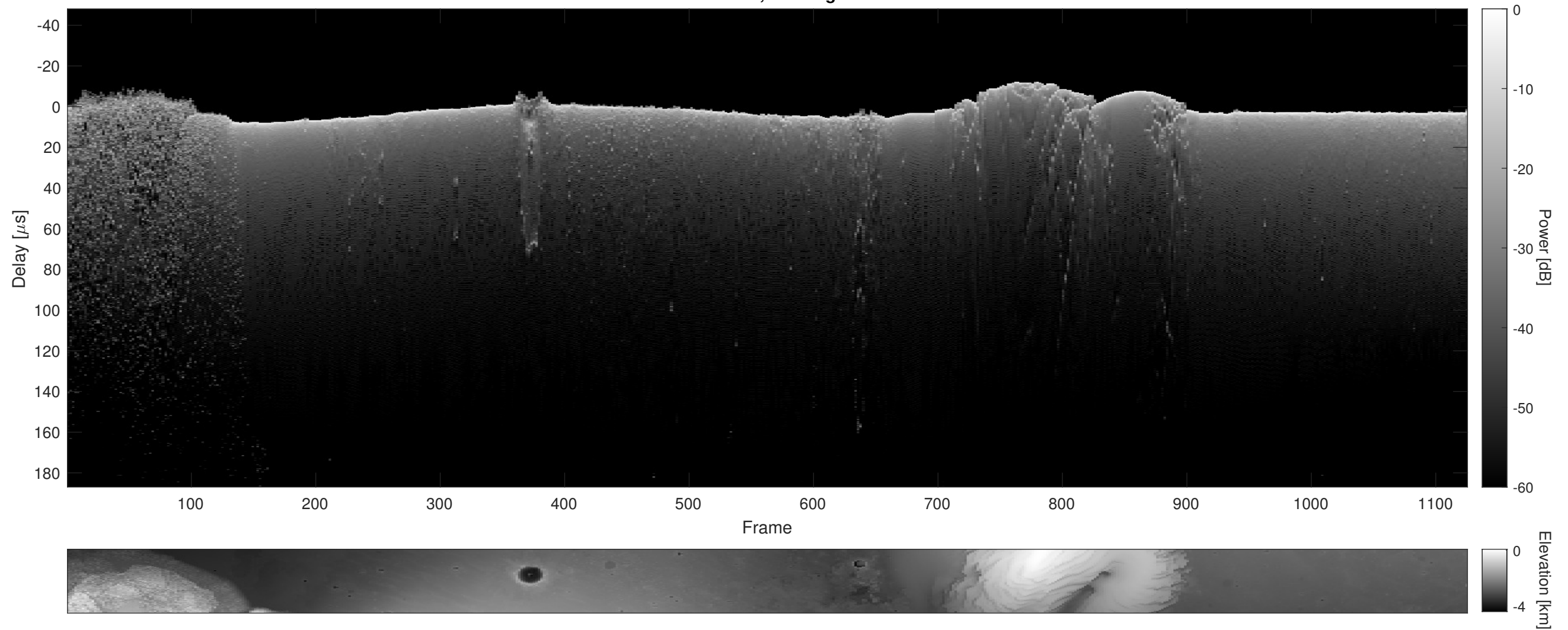
Orbit 11991, Cluttergram
