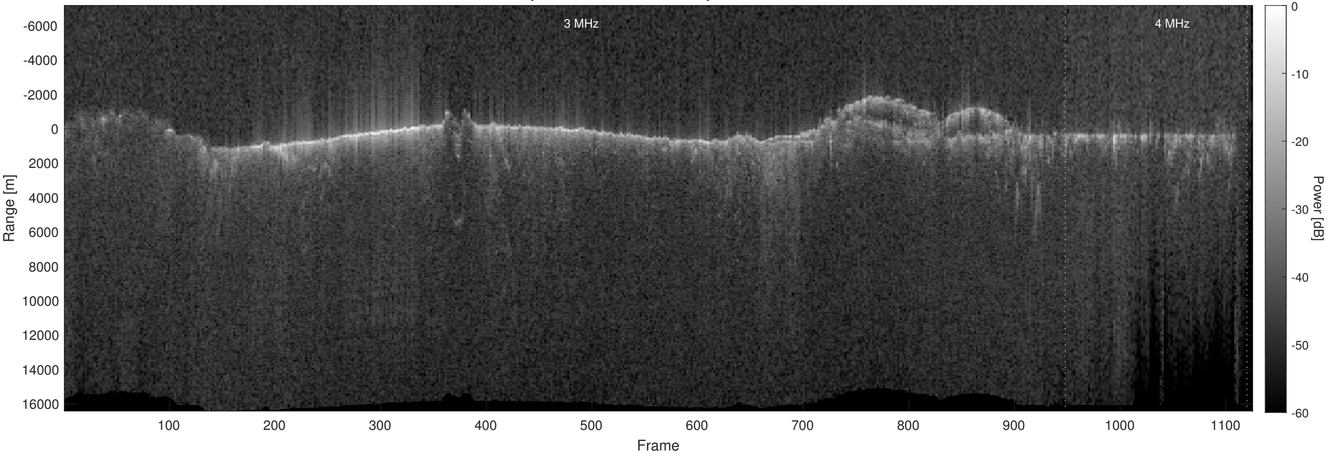
Orbit 11991, Optimized, No Window, Depth-Corrected, Channel 2
