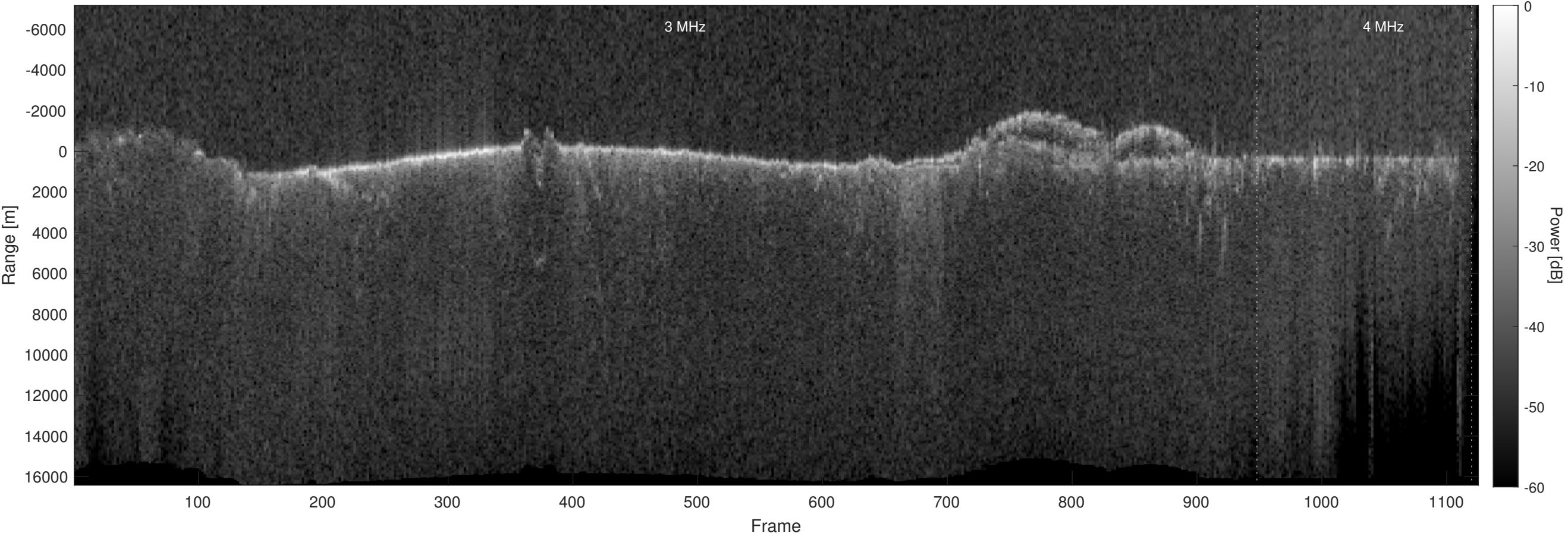
Orbit 11991, Optimized, Window, Depth-Corrected, Channel 2
