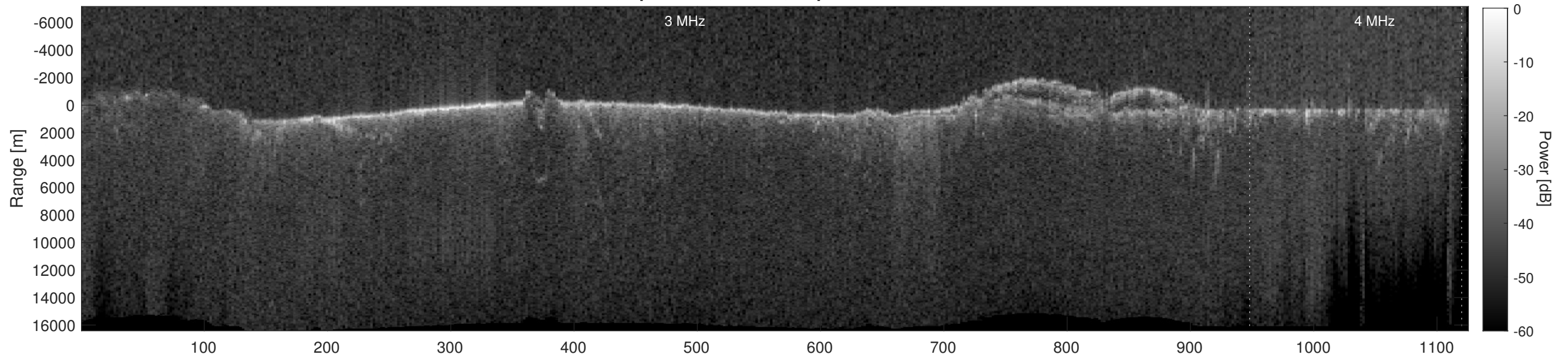
Orbit 11991, Depth-Corrected Cluttergram
