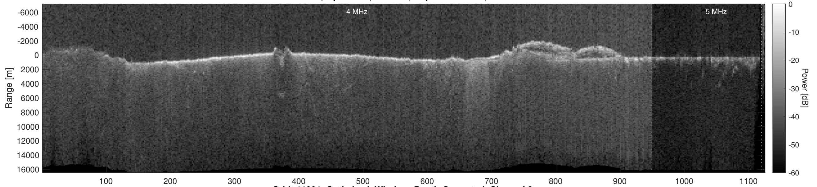
Orbit 11991, Optimized, Window, Depth-Corrected, Channel 2
