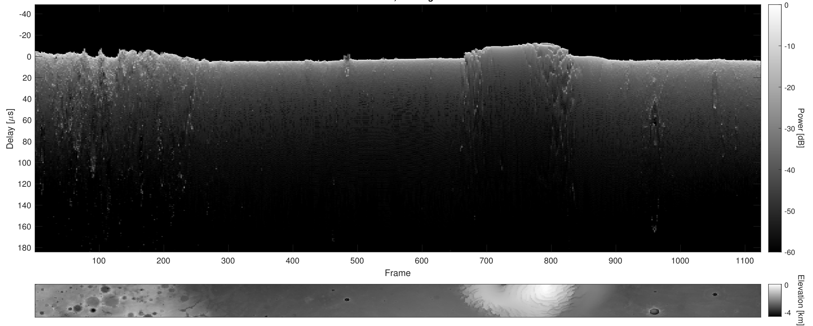
Orbit 11993, Cluttergram
