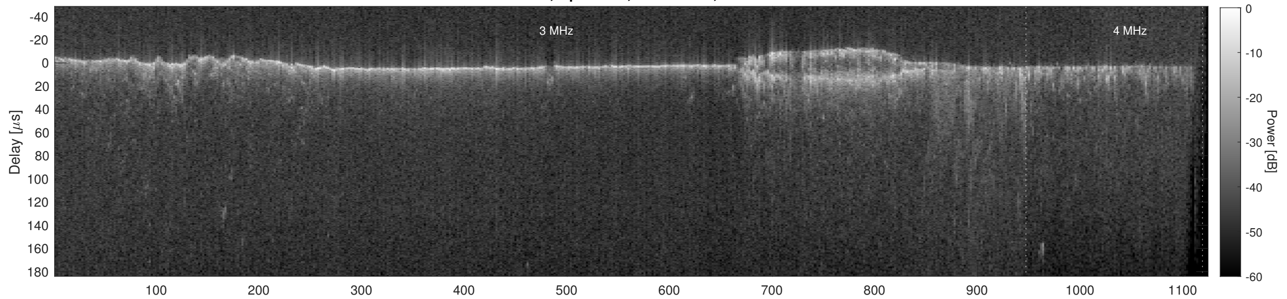
Orbit 11993, Cluttergram
