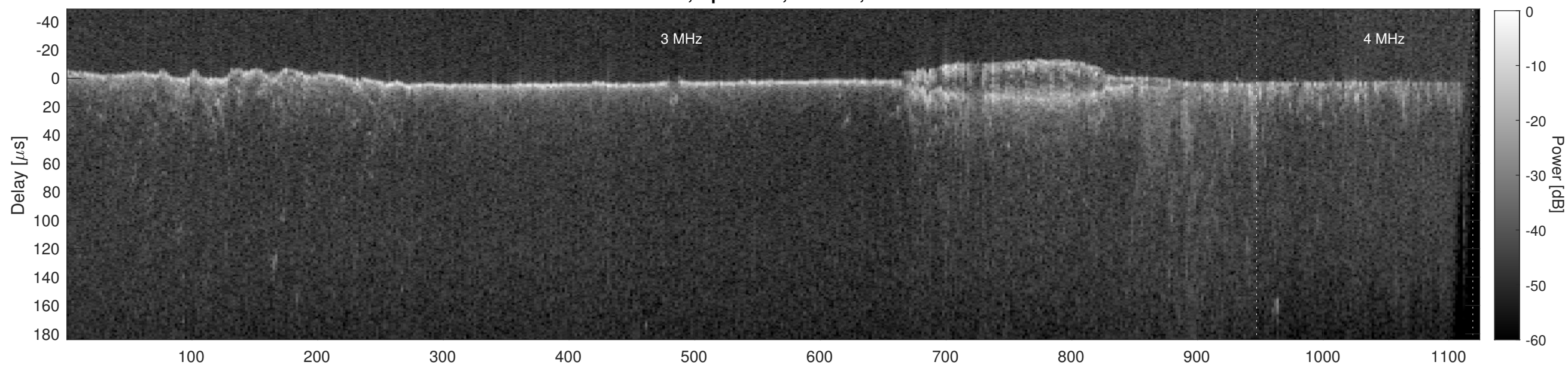
Orbit 11993, Cluttergram
