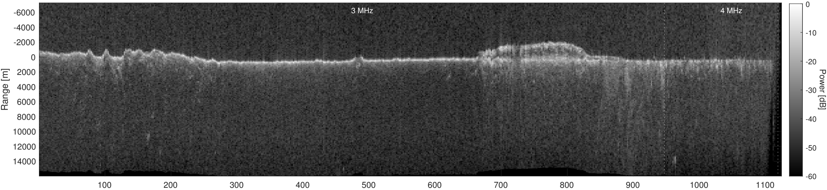
Orbit 11993, Depth-Corrected Cluttergram
