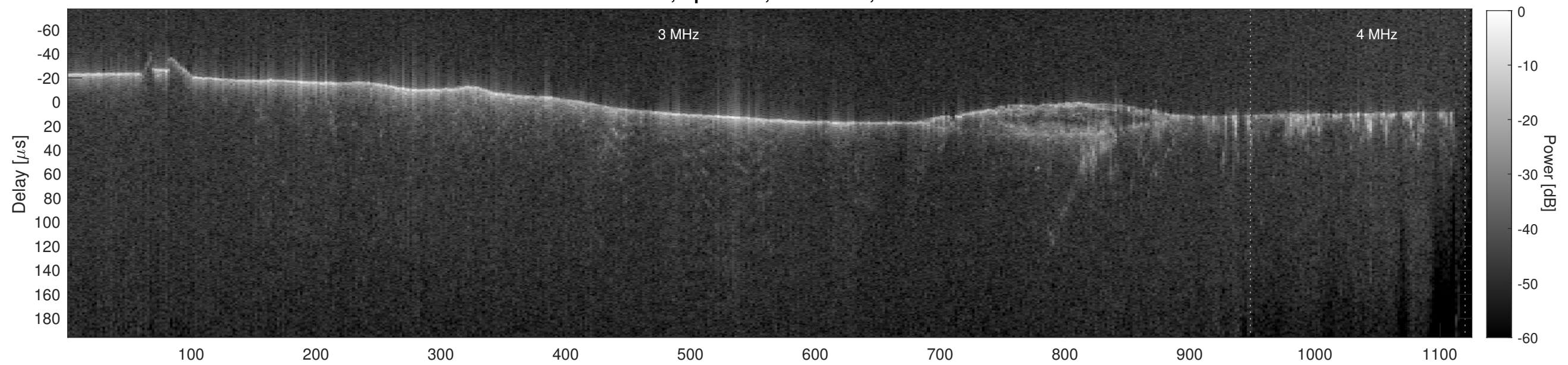
Orbit 11994, Cluttergram
