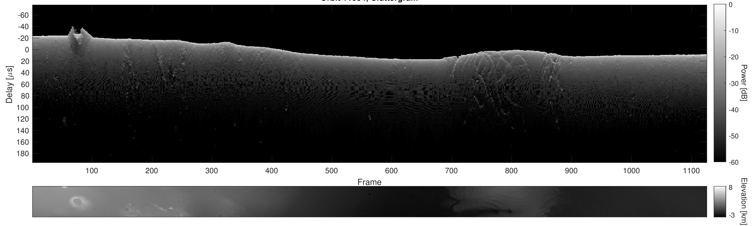
Orbit 11994, Cluttergram
