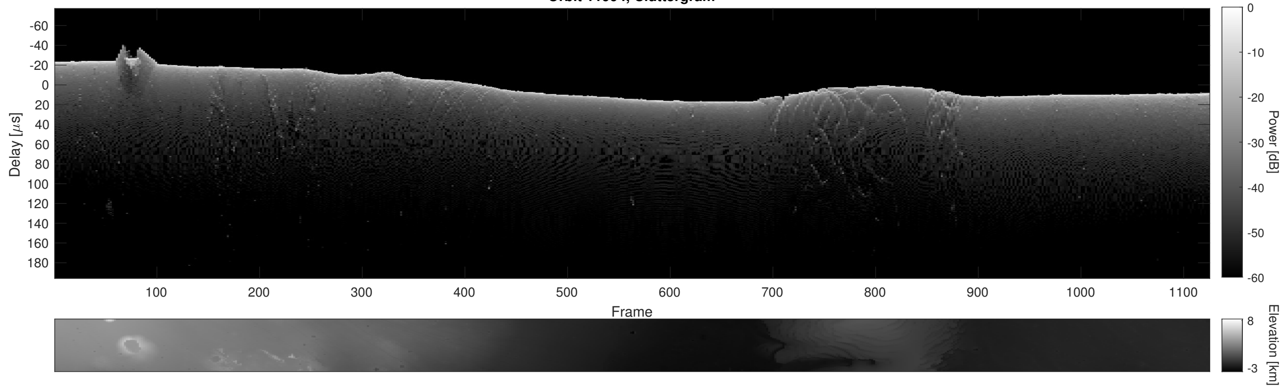
Orbit 11994, Cluttergram
