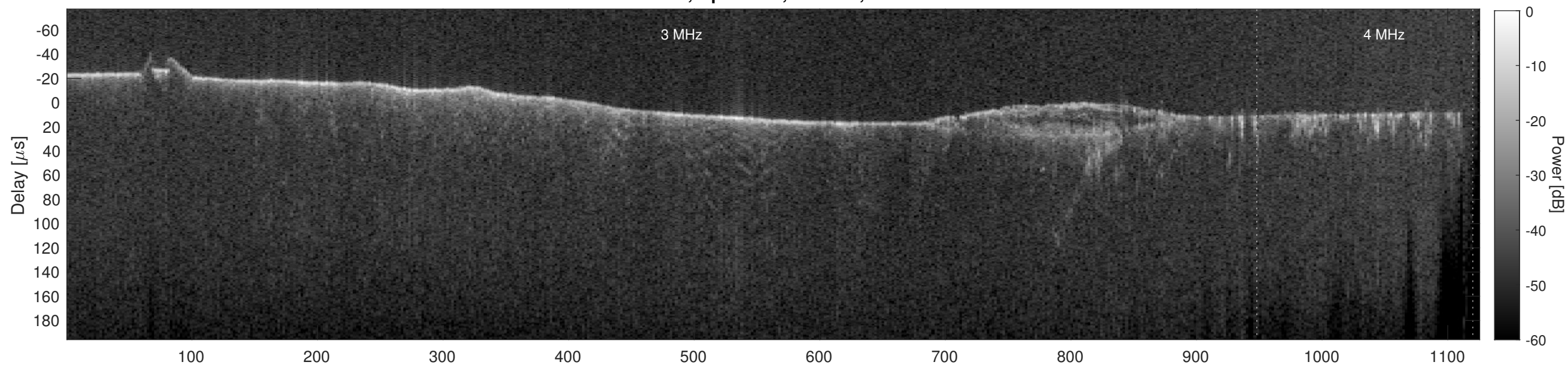
Orbit 11994, Cluttergram
