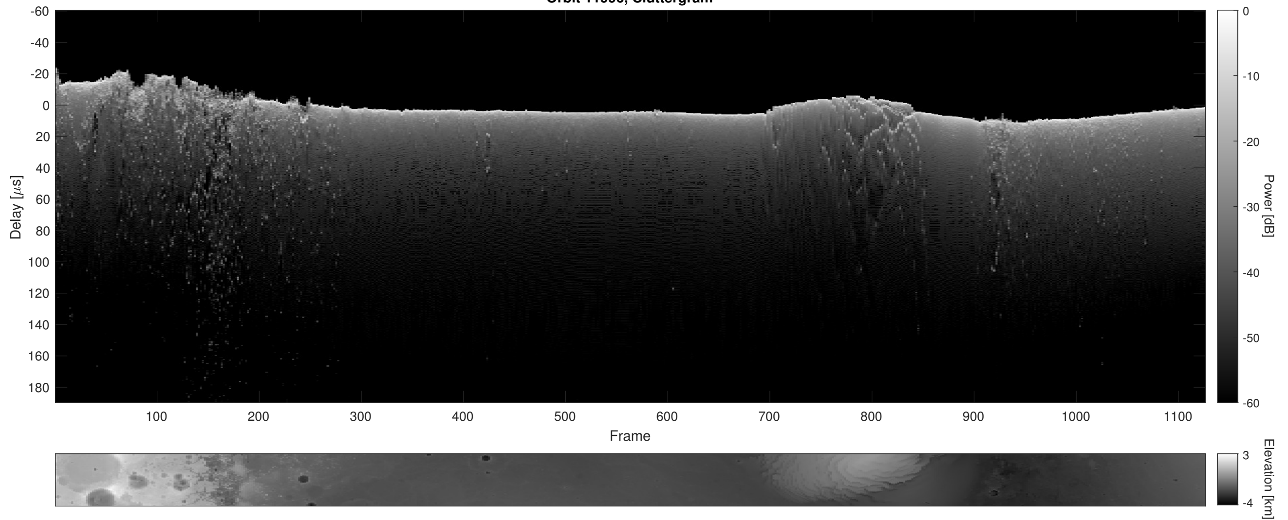
Orbit 11996, Cluttergram
