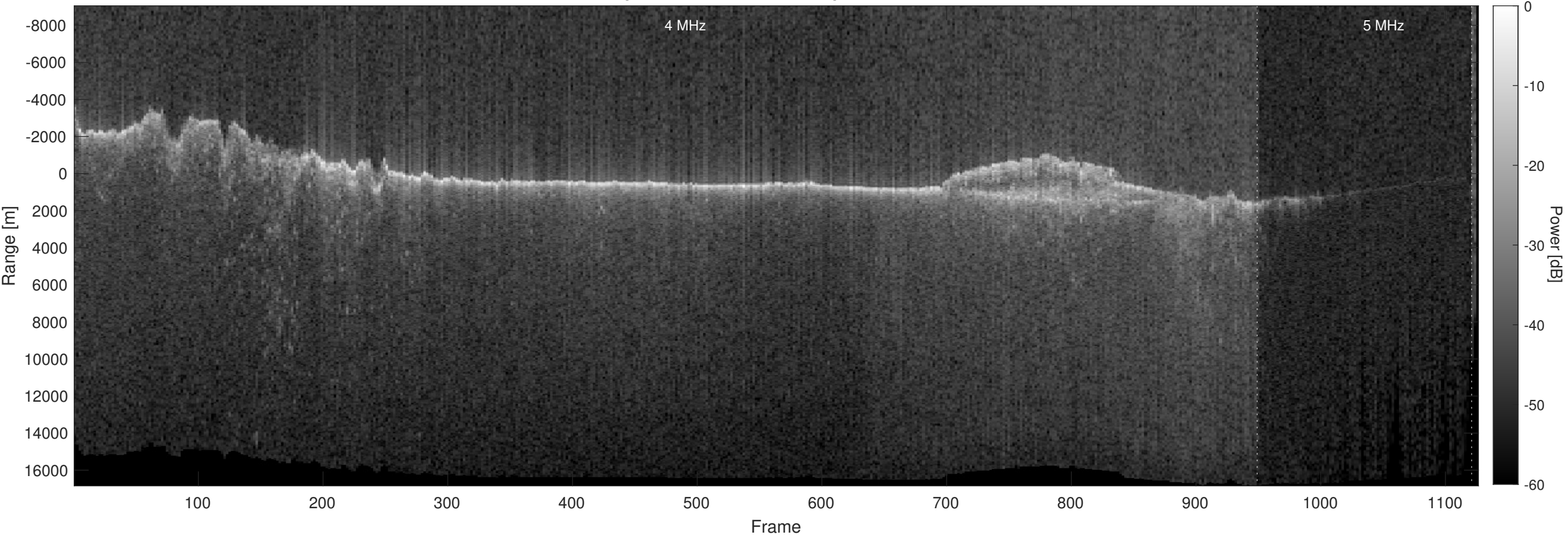
Orbit 11996, Optimized, No Window, Depth-Corrected, Channel 2
