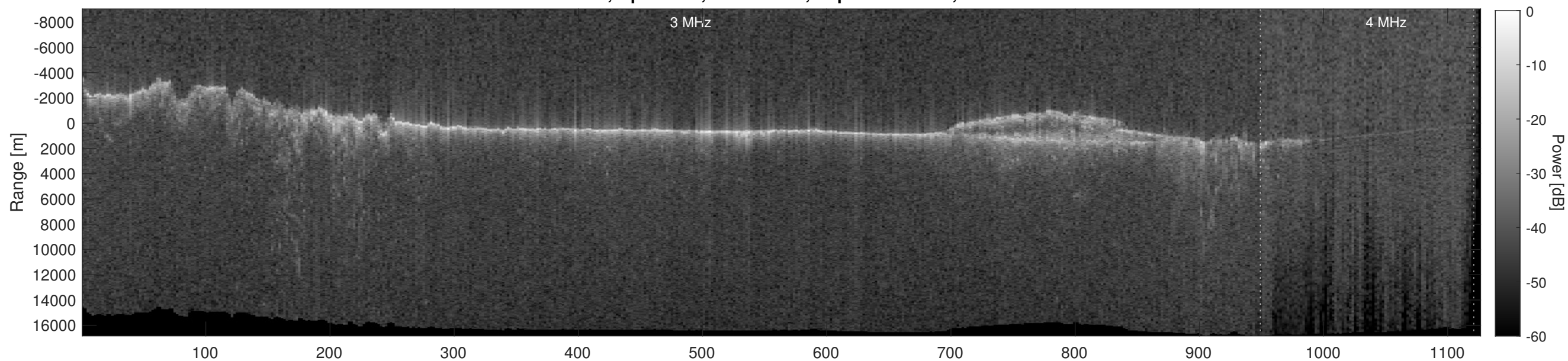
Orbit 11996, Depth-Corrected Cluttergram
