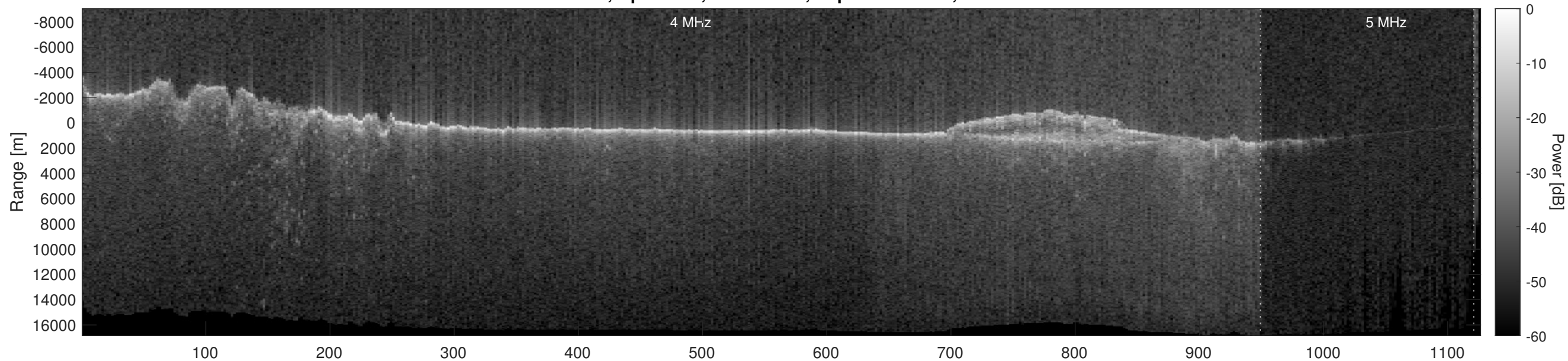
Orbit 11996, Optimized, No Window, Depth-Corrected, Channel 2
