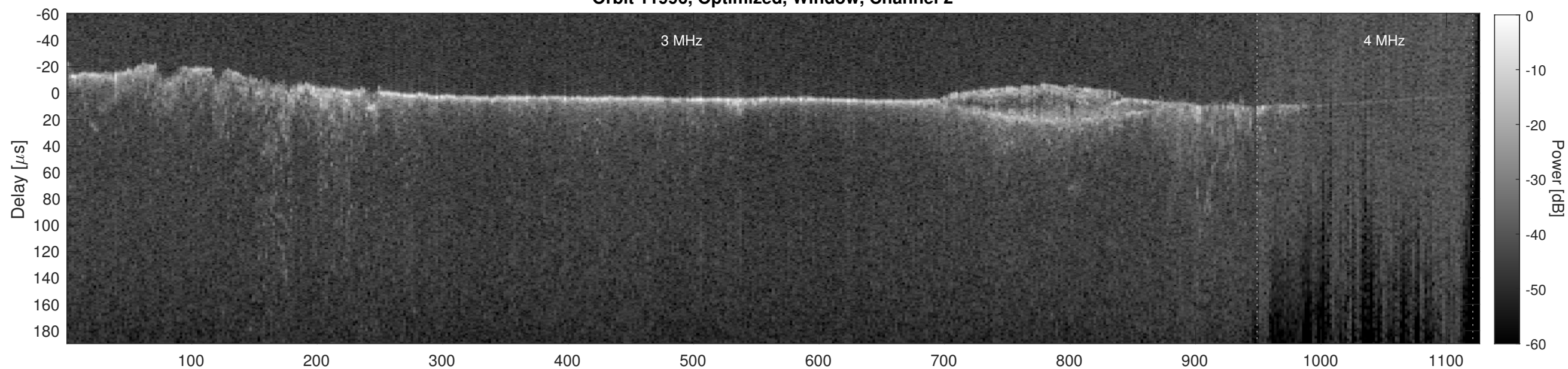
Orbit 11996, Cluttergram
