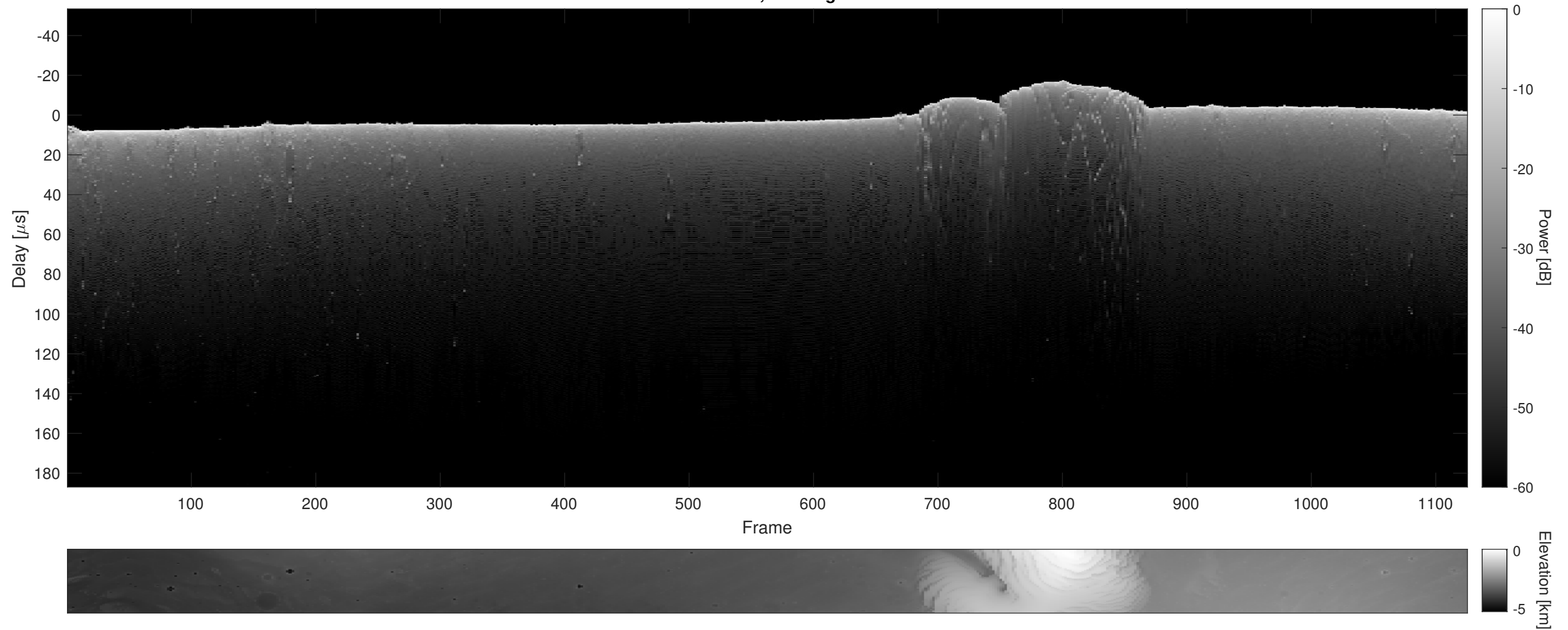
Orbit 11997, Cluttergram
