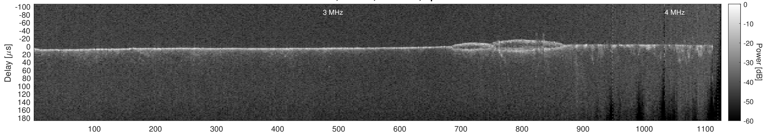
Orbit 11997, Cluttergram
