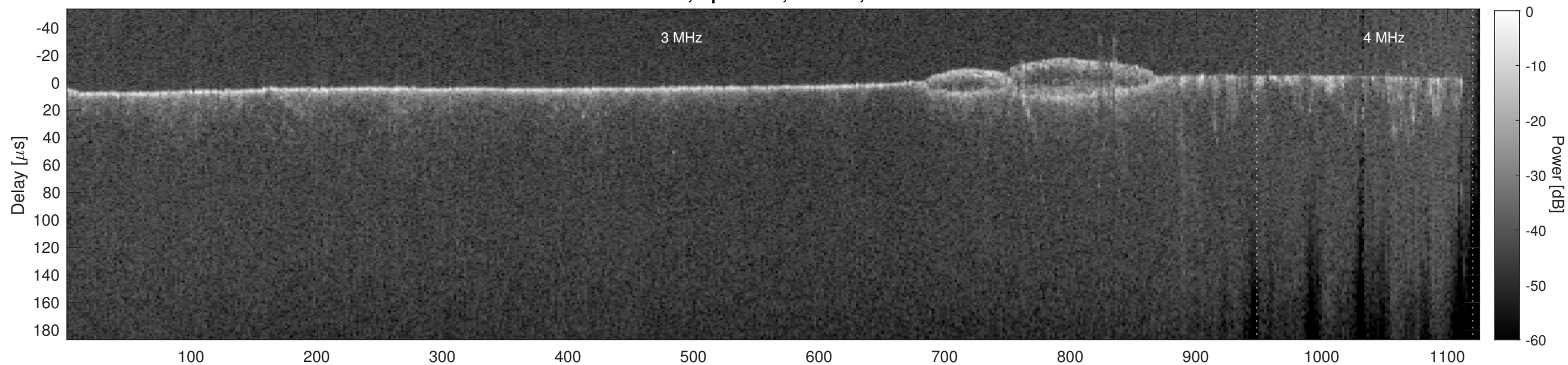
Orbit 11997, Cluttergram
