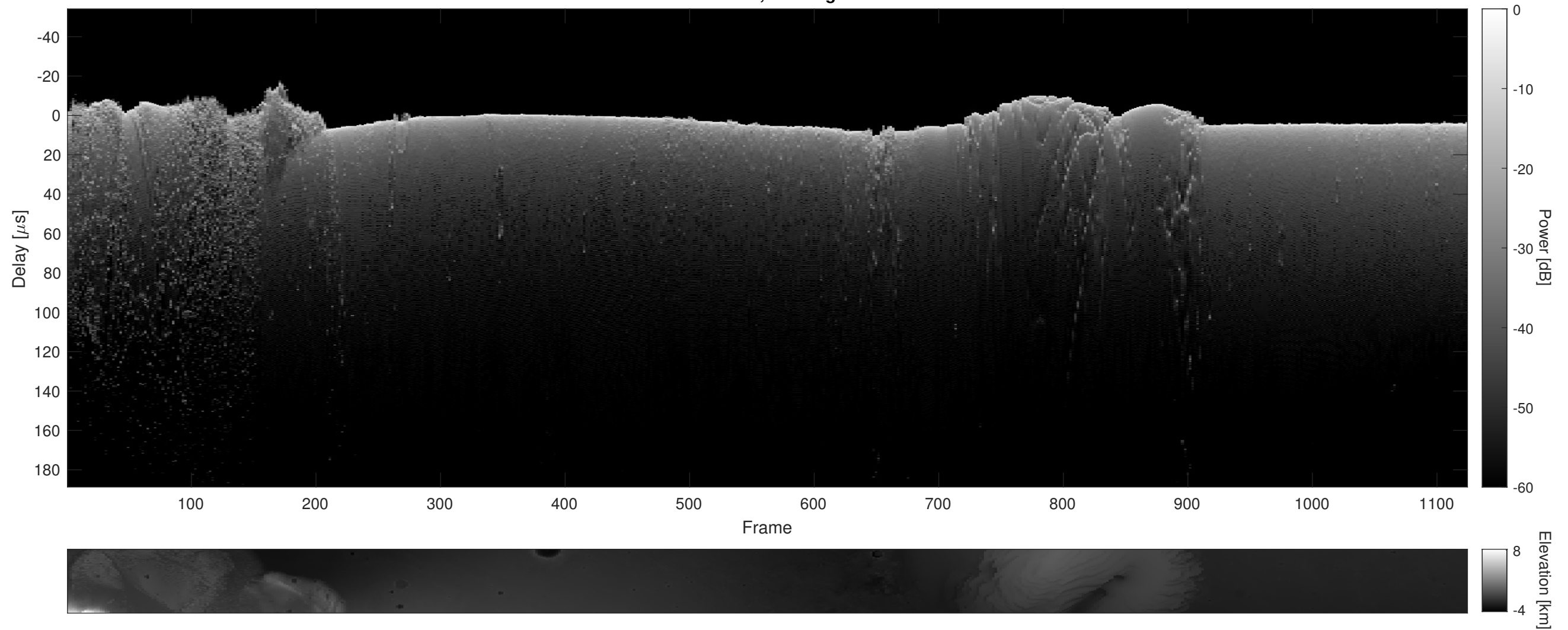
Orbit 11998, Cluttergram
