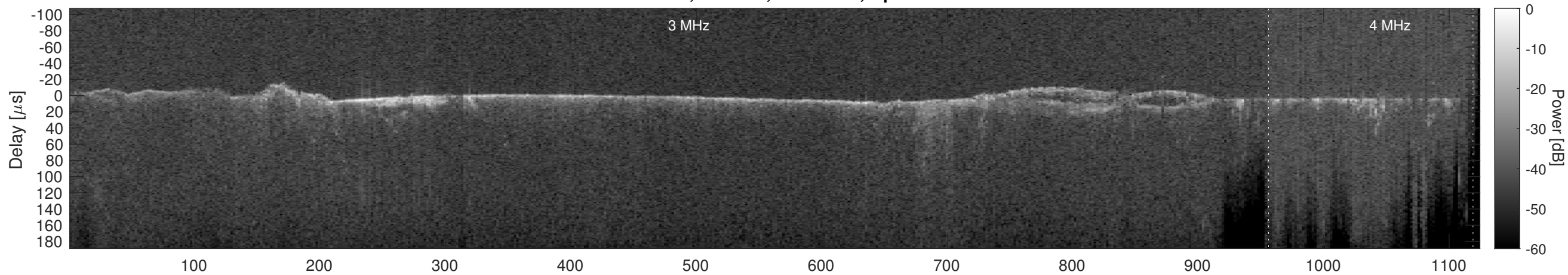
Orbit 11998, Cluttergram
