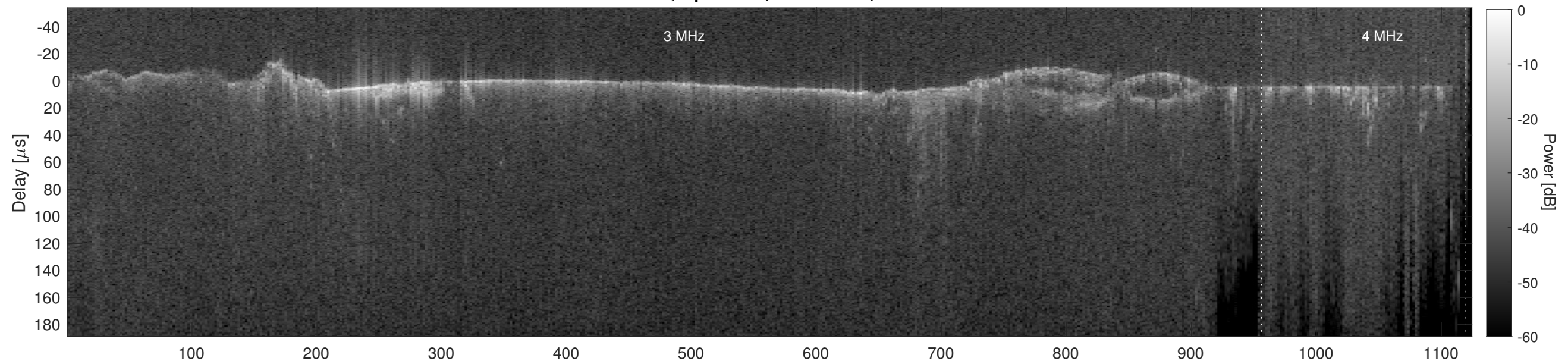
Orbit 11998, Cluttergram
