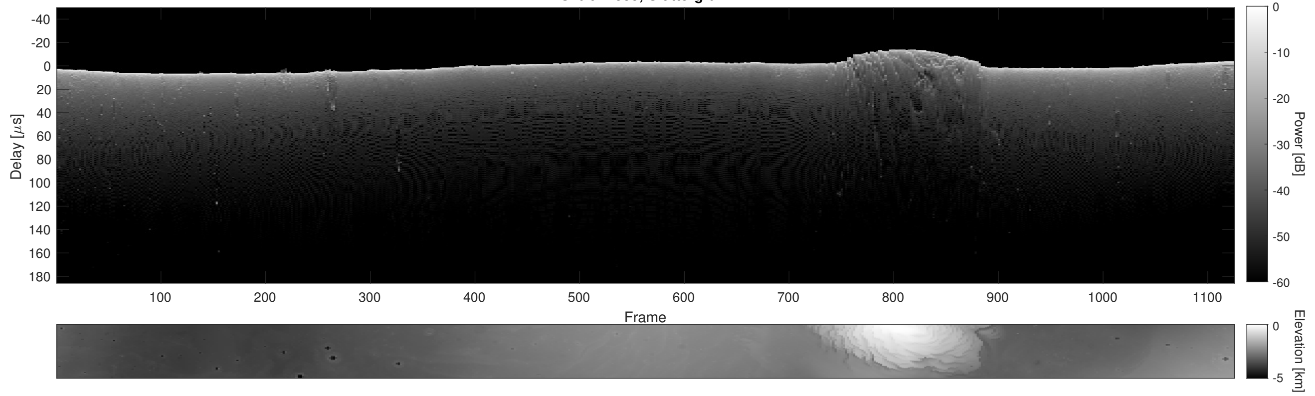
Orbit 11999, Cluttergram
