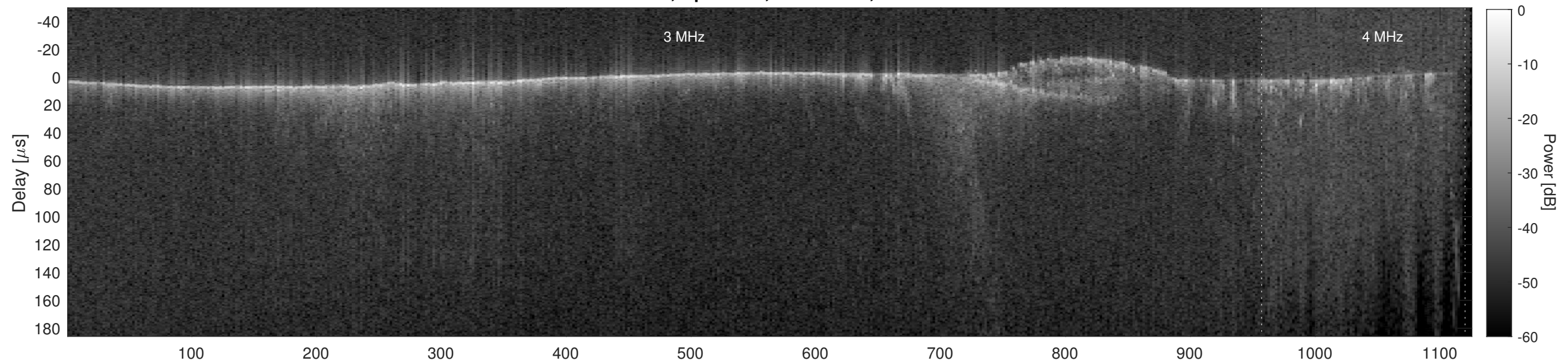
Orbit 11999, Cluttergram
