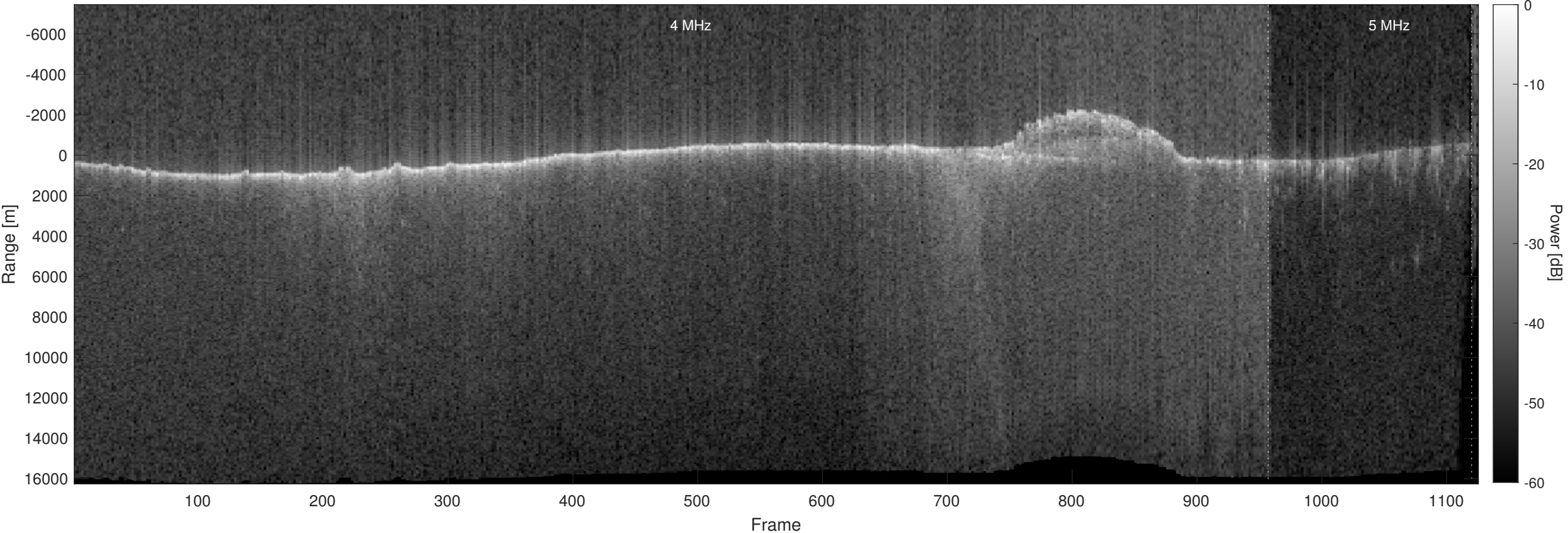
Orbit 11999, Optimized, No Window, Depth-Corrected, Channel 2
