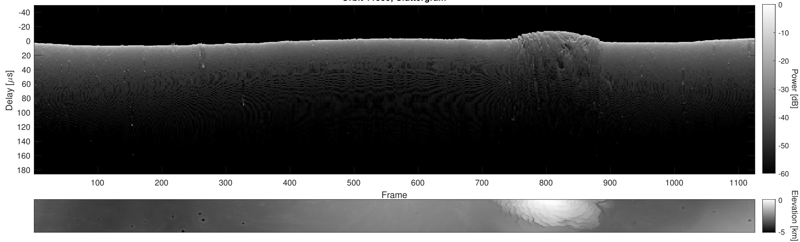
Orbit 11999, Cluttergram
