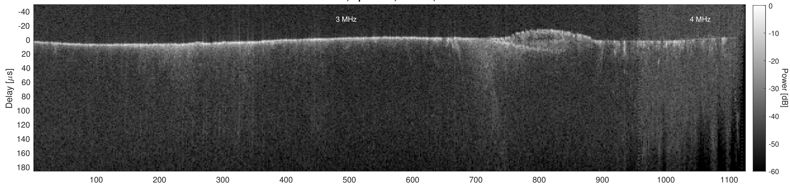
Orbit 11999, Cluttergram
