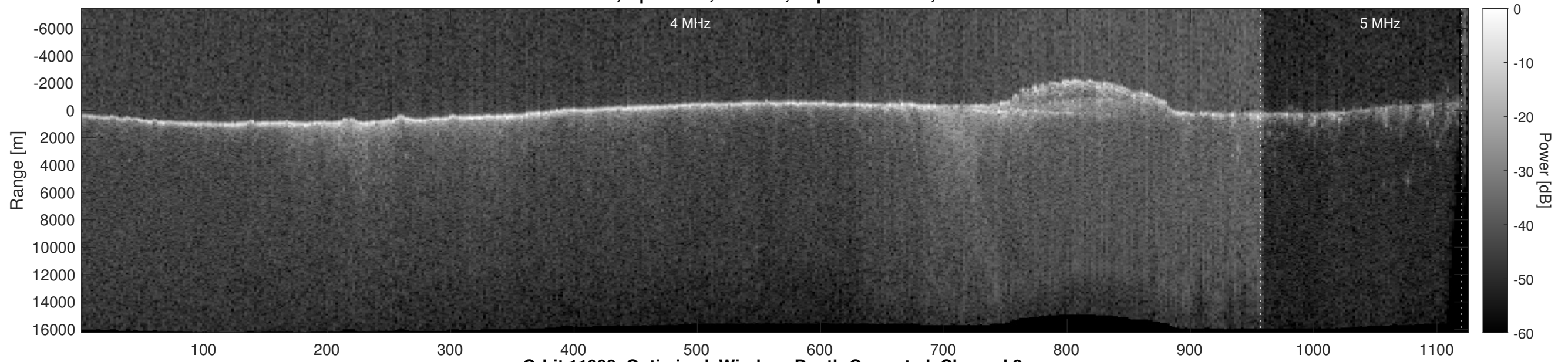
Orbit 11999, Optimized, Window, Depth-Corrected, Channel 2
