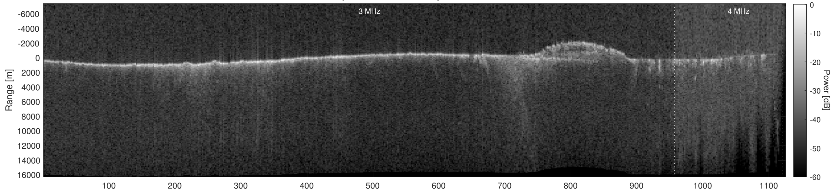
Orbit 11999, Depth-Corrected Cluttergram
