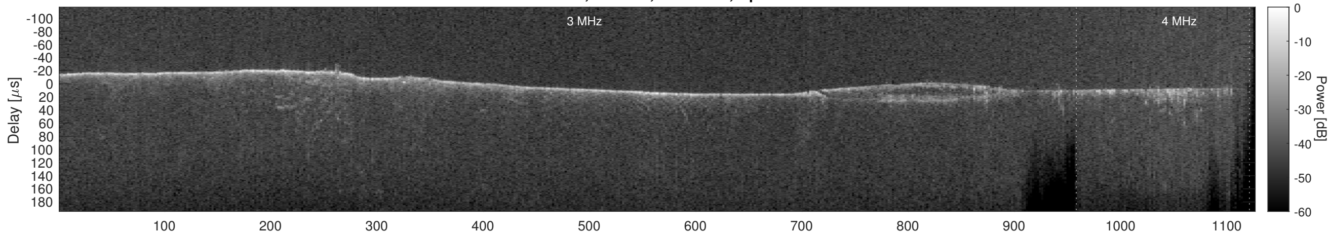
Orbit 12001, Cluttergram
