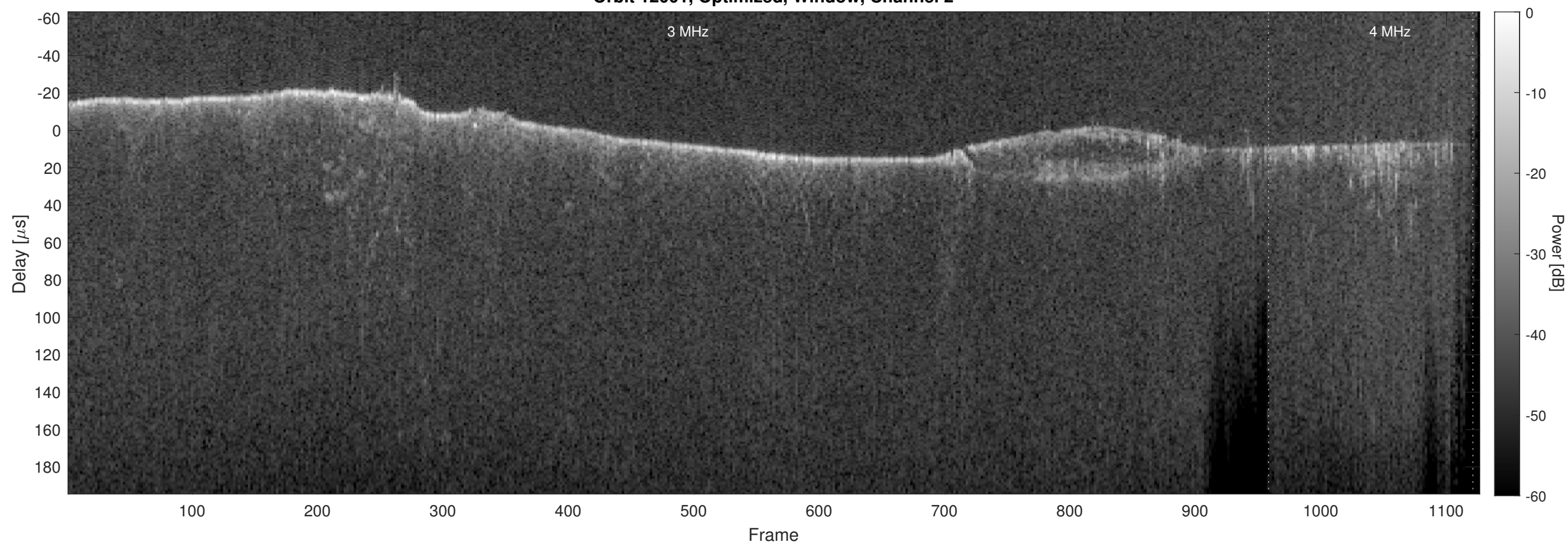
Orbit 12001, Optimized, Window, Channel 2
