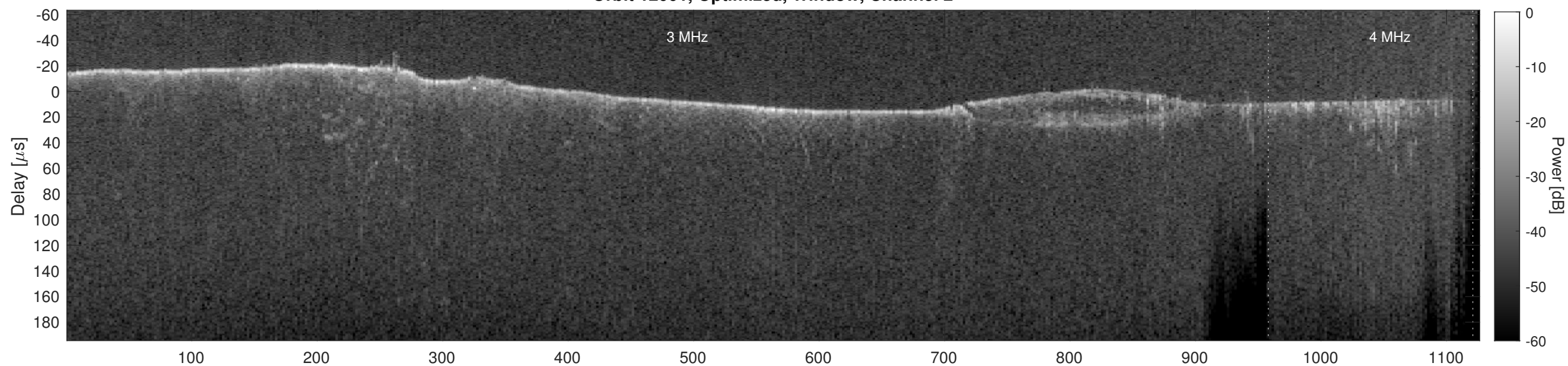
Orbit 12001, Cluttergram
