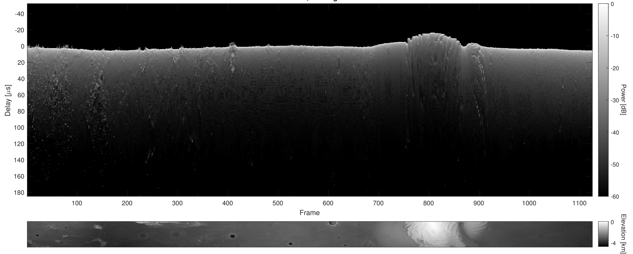
Orbit 12002, Cluttergram
