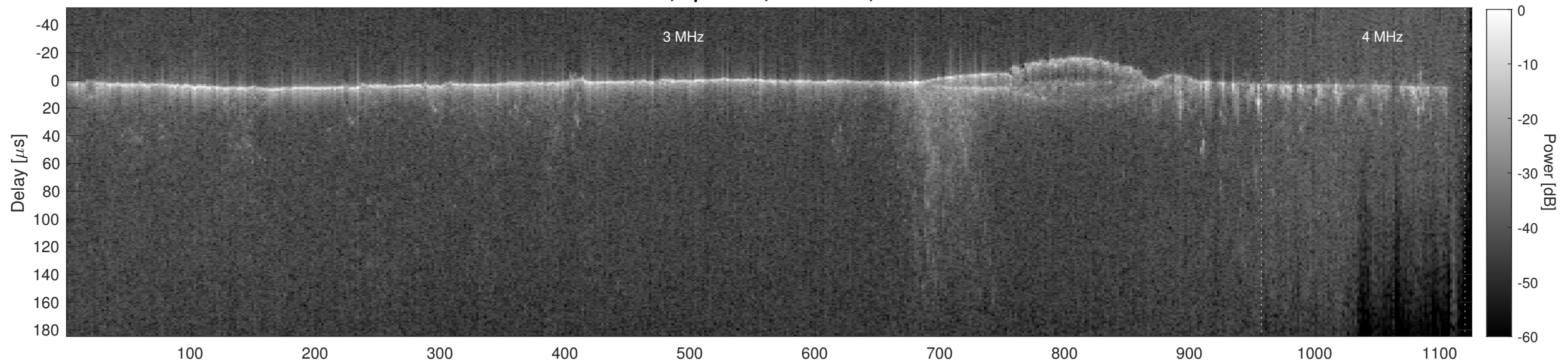
Orbit 12002, Cluttergram
