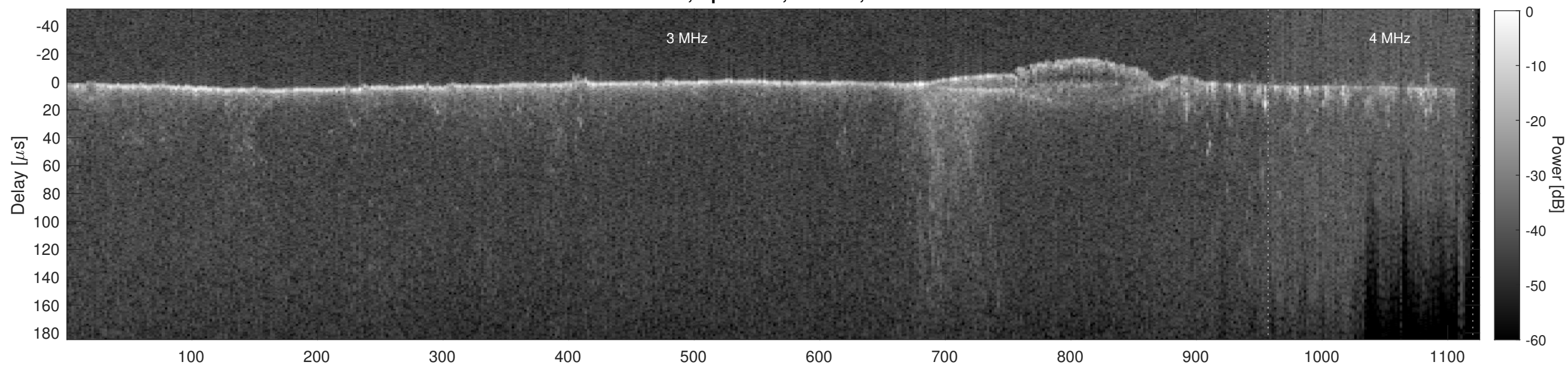
Orbit 12002, Cluttergram
