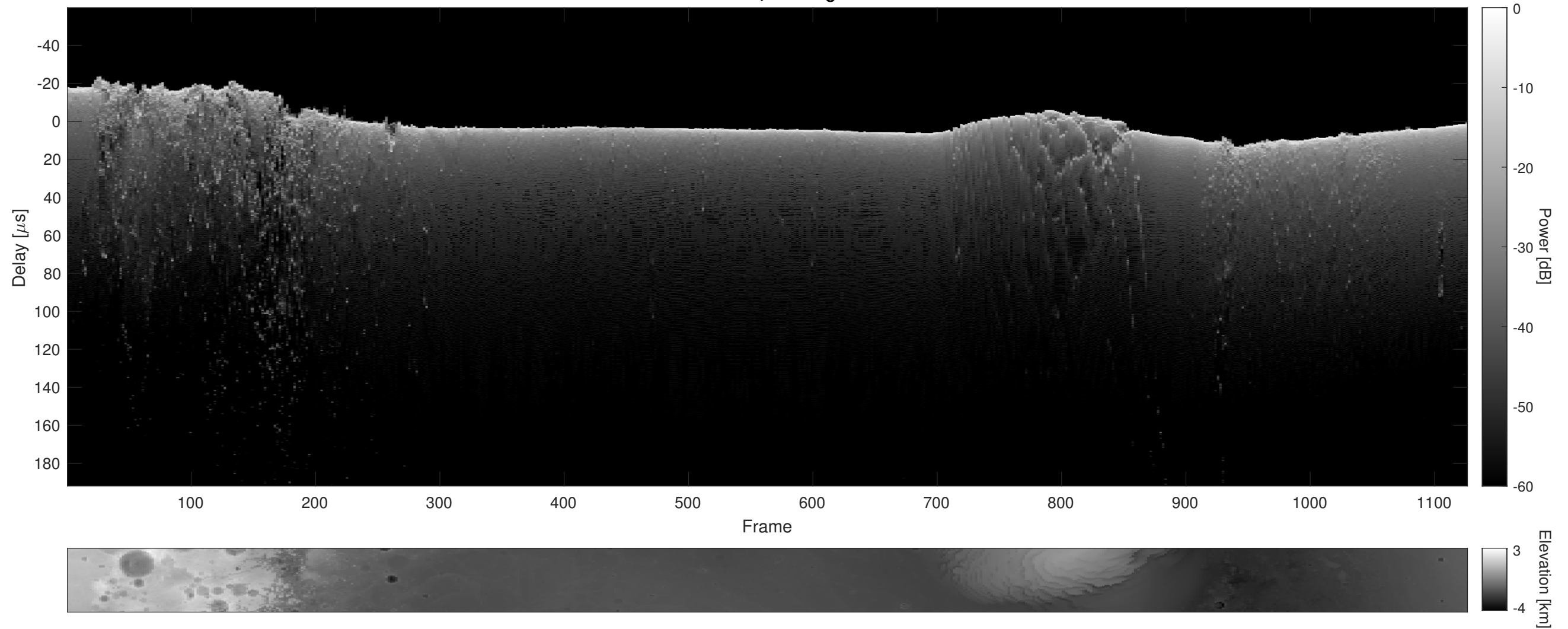
Orbit 12003, Cluttergram
