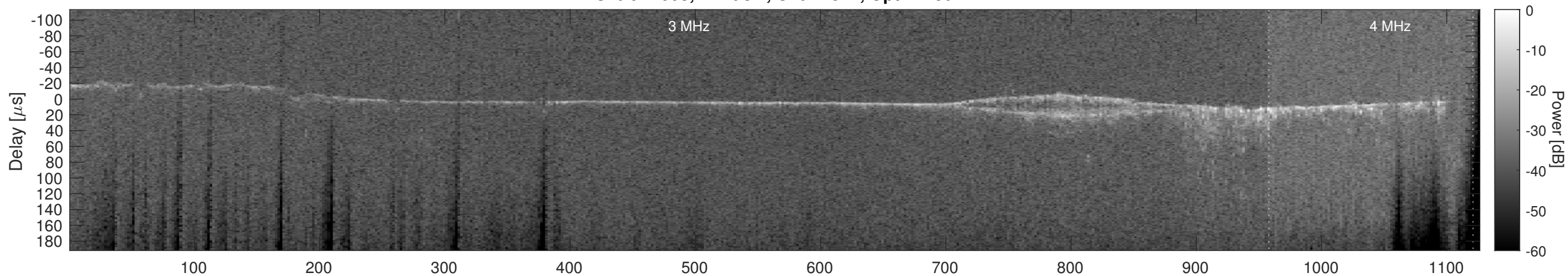
Orbit 12003, Cluttergram
