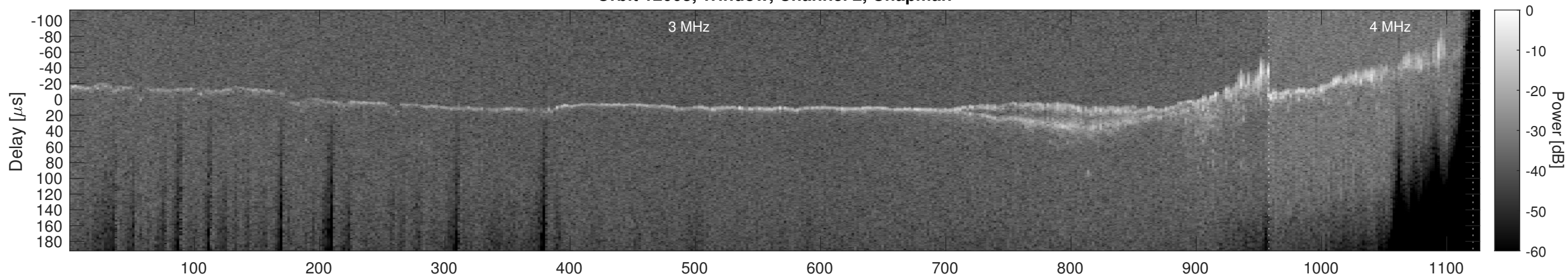
Orbit 12003, Window, Channel 2, Optimized
