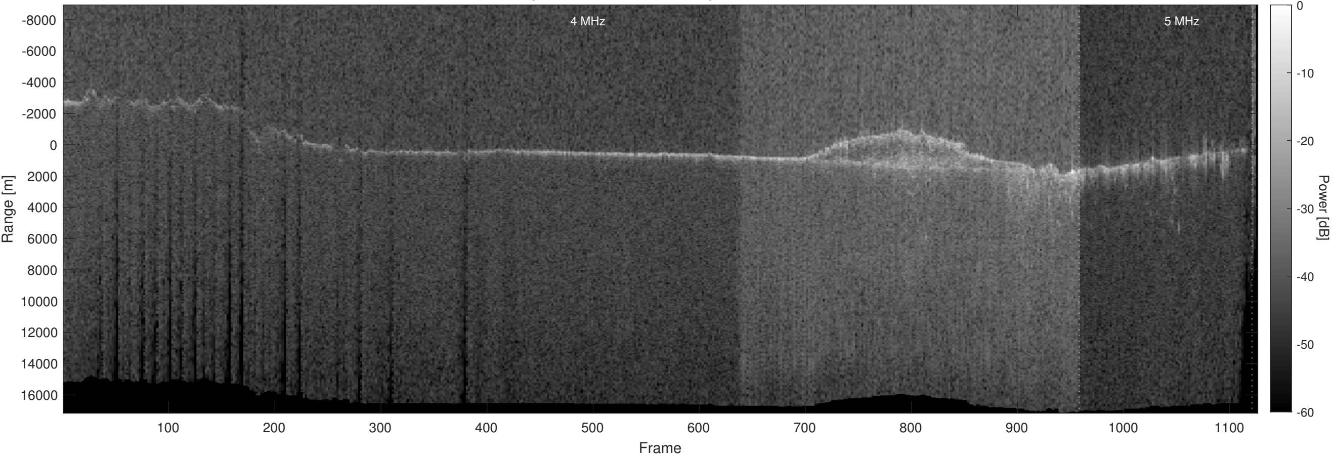
Orbit 12003, Optimized, No Window, Depth-Corrected, Channel 2
