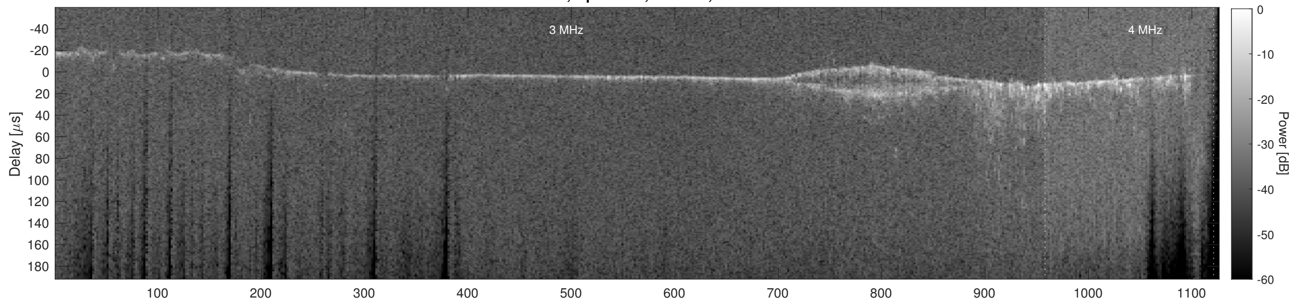
Orbit 12003, Cluttergram
