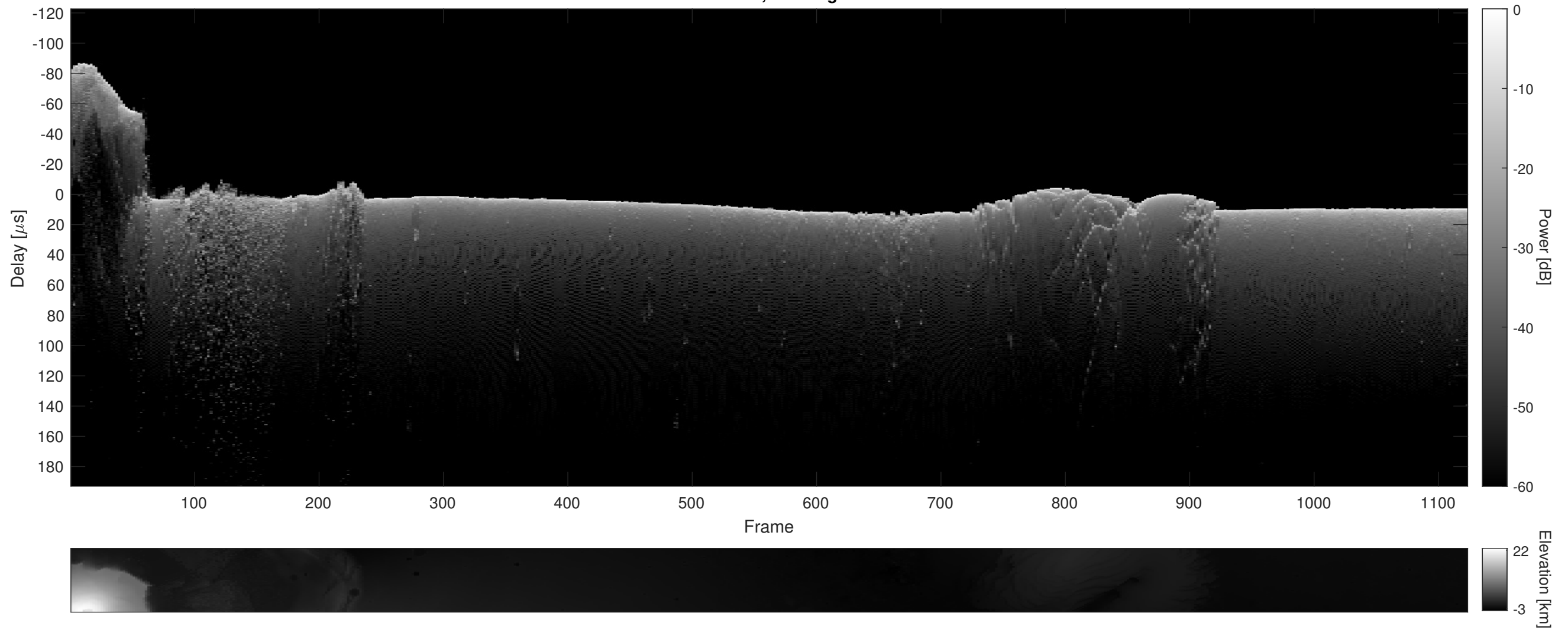
Orbit 12005, Cluttergram
