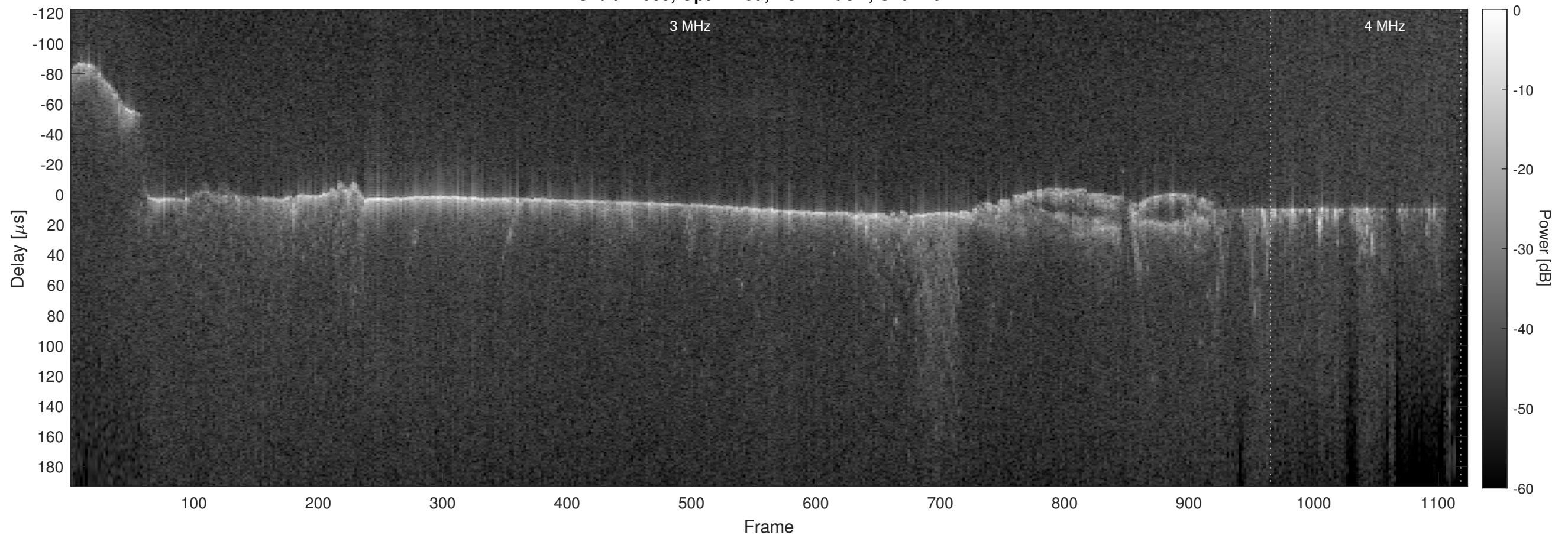
Orbit 12005, Optimized, No Window, Channel 2
