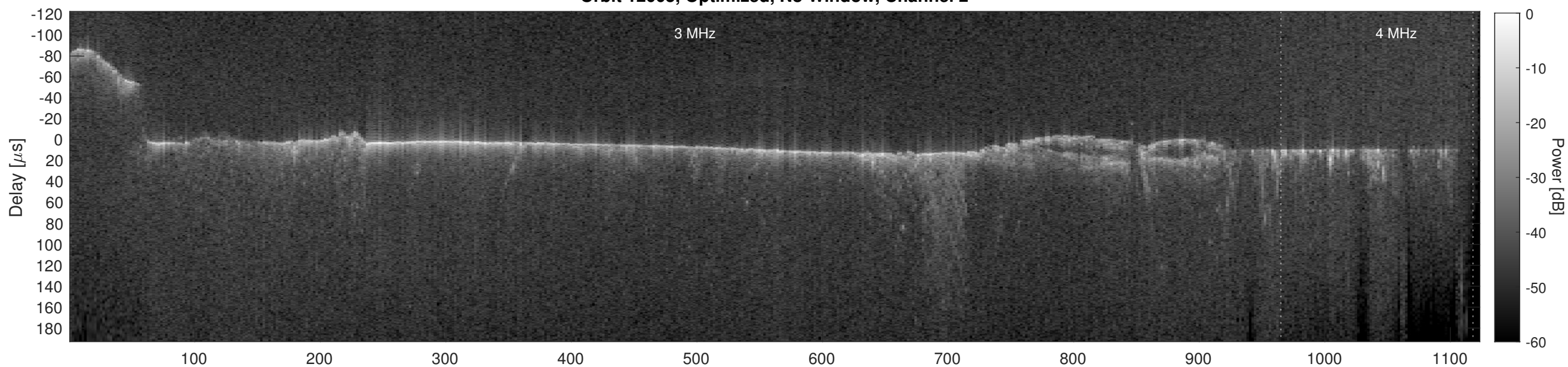
Orbit 12005, Cluttergram
